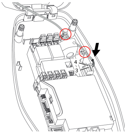
Fig. 13: Tilkobling Downgrade-inngang
