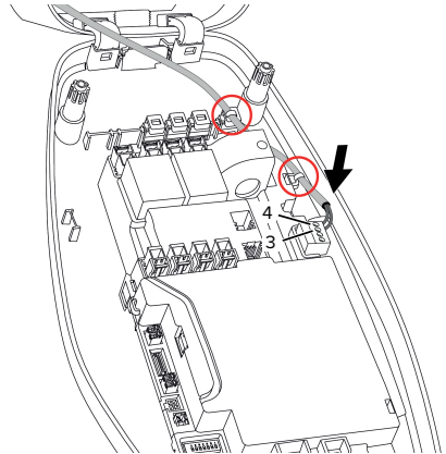
Fig. 13: Downgrade input connection
