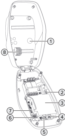
Fig. 3: Vista interior
