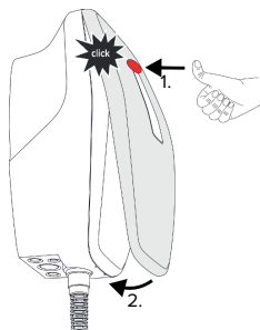
Fig. 17: Colocar o painel frontal - 1
